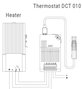
Connection example
