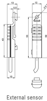
External sensor
