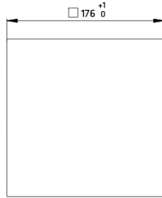
Enclosure cut-out
