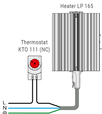
Connection example
